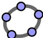
GeoGebra Classic 6
